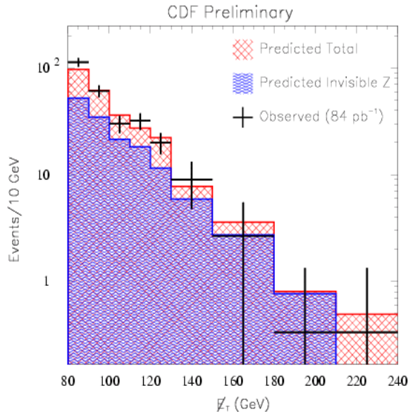
Figure 1: Distribution of \cancel{E}_T in jets + \cancel{E}_T events in CDF Run I data.
