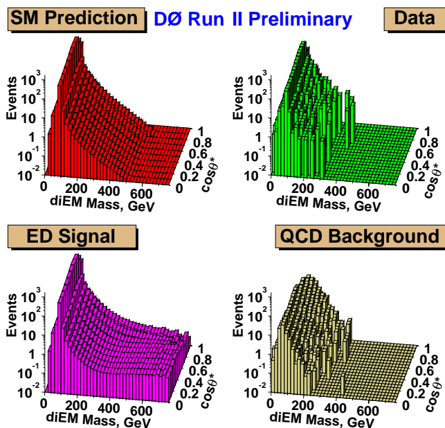
Figure 2: Distributions of invariant mass of electron and photon pairs versus scattering angle in DØ Run II data for (top-left) Standard Model expectation, (top-right) data, (bottom-left) Standard Model plus an extra dimensions signal, and (bottom-right) QCD background.
