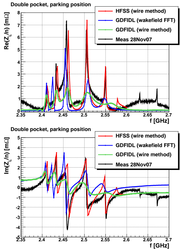
Figure 2: Longitudinal impedance of a FP420 double-pocket pipe in parking position calculated with simulations (HFSS and GDFIDL) and compared to laboratory experiments.
